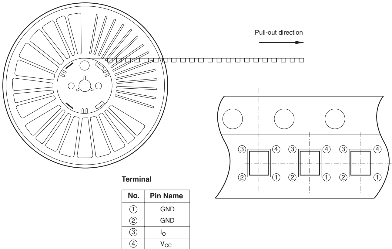
Fig. 4 Product Insertion Direction
