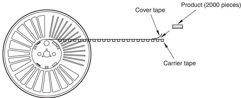
Fig. 5 Inner Packing
