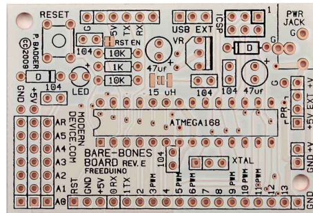
A BBB pcb board shown actual size, for comparison purposes.
