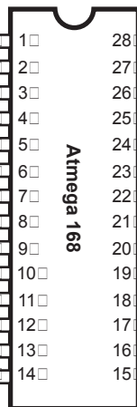
Pin mapping of the Atmega168 / 238 chip to the BBB (Arduino)
